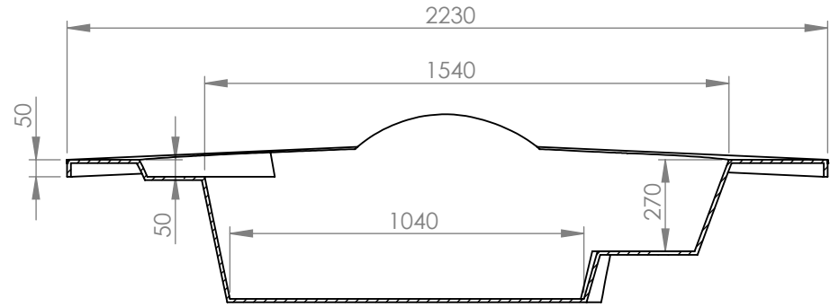
SECTION B-B
