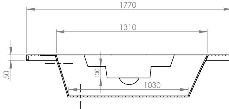
SECTION B-B
